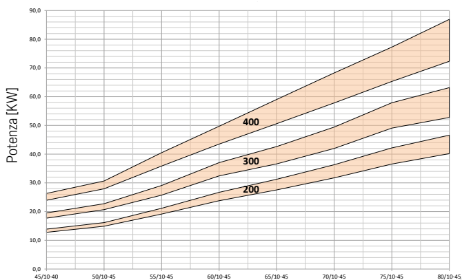
Temperature PRIMARIO/SECONDARIO IN-OUT [°C]
